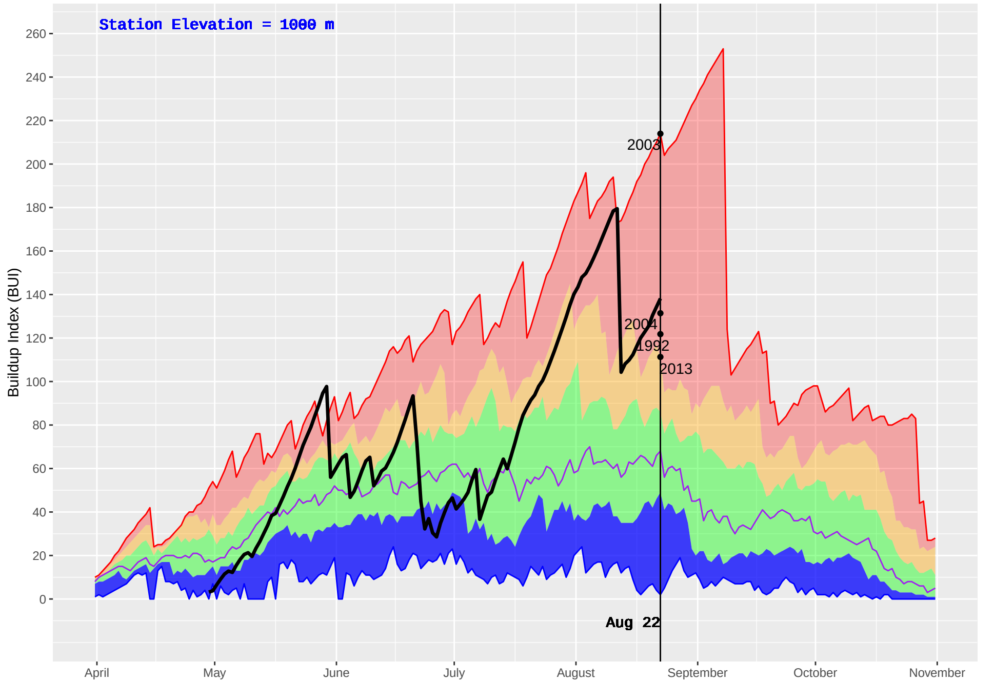
SUCCOUR CREEK (374) : Historical (1986–2016) and Current (2018) Daily Buildup Index (BUI)
