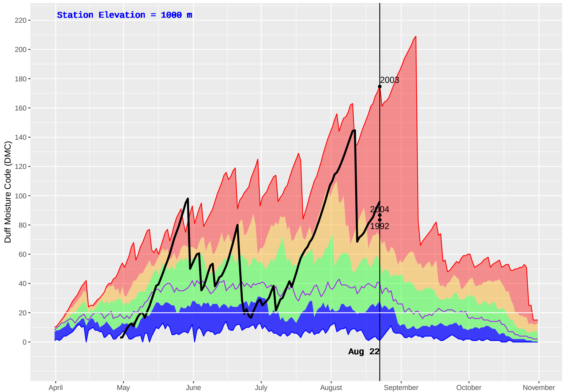
SUCCOUR CREEK (374) : Historical (1986–2016) and Current (2018) Daily Duff Moisture Code (DMC)
